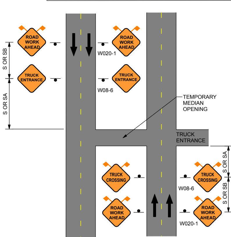
Truck Crossing or Entrance
