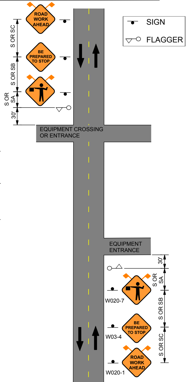
Equipment Crossing or Entrance on Undivided Highway
